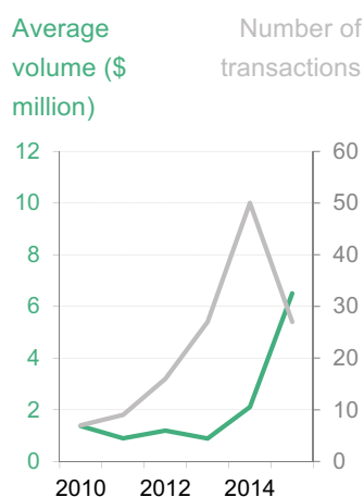
Figure 56: Transaction statistics
